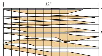
1/8" Plywood Wing Saddle & Longerons (make four sets)
